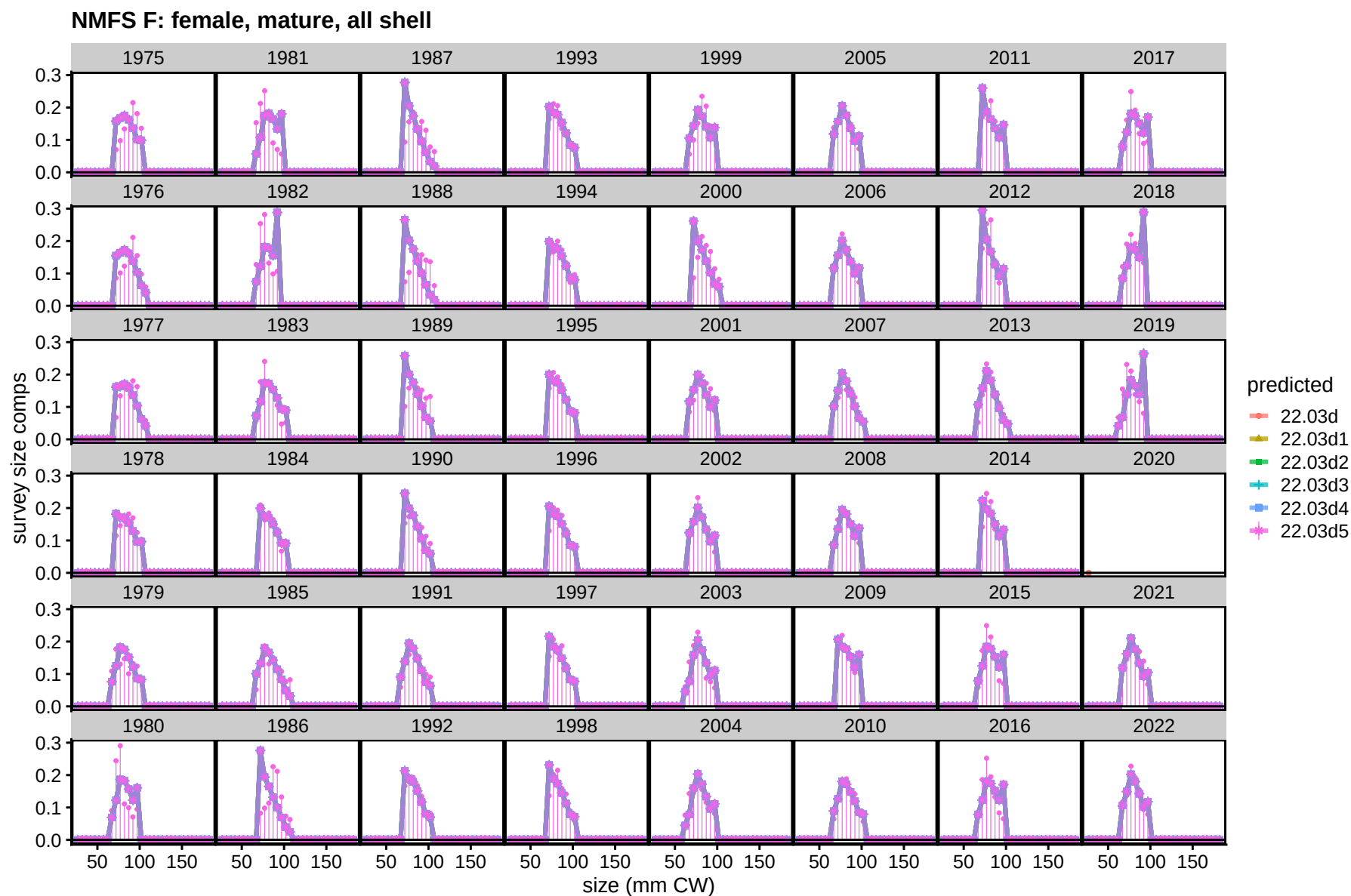
Figure 111. TCSAM02 models fits to survey size compositions in the NMFS F survey. Preferred model is 22.03d5.
