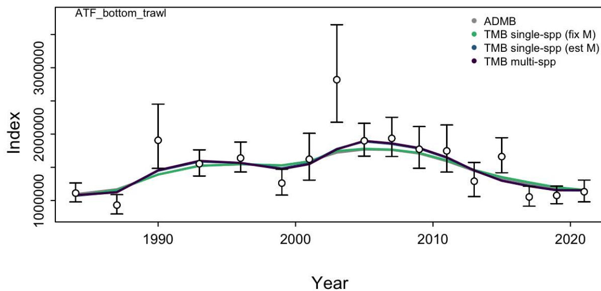
Figure 7A.8. Observed (circles) and expected (lines) AFSC trawl survey biomass across the ADMB model and CEATTLE single- and multi-species models.
