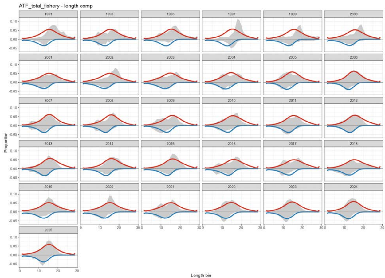
Figure 7.21c: Fits to annual age and length compositions for the bottom trawl survey (top) and fishery (bottom) observed and expected (lines) size/age-composition data for Model 25.1. Females are red and males are blue.
