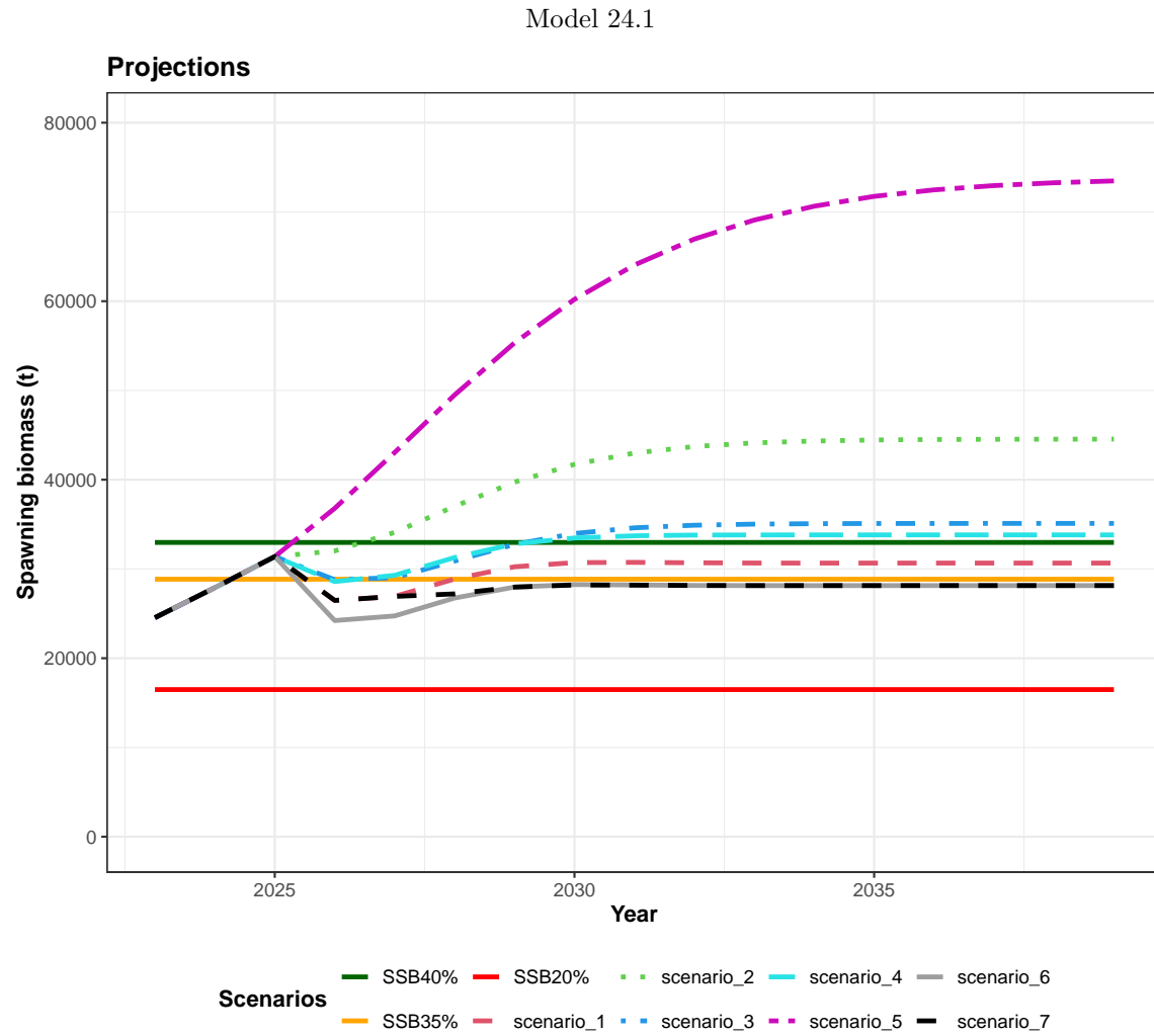
Figure 2A.40: Projected spawning stock biomass under seven NPFMC projection scenarios for Model 24.1.
