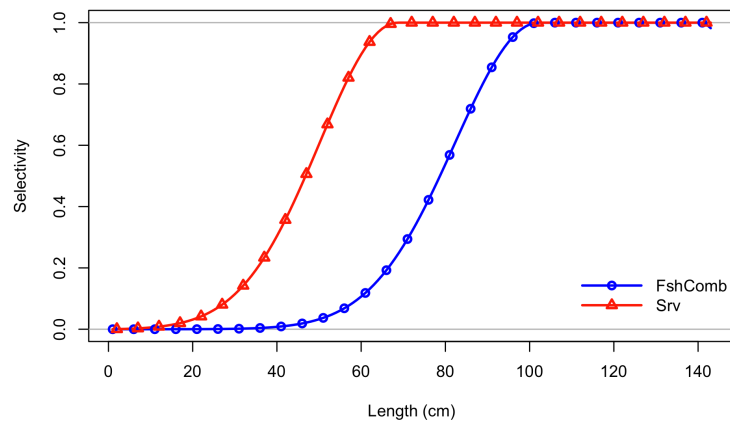
Figure 2A.9: Survey and fishery selectivity curves for Models 24.1, 24.1a, and 24.0.
