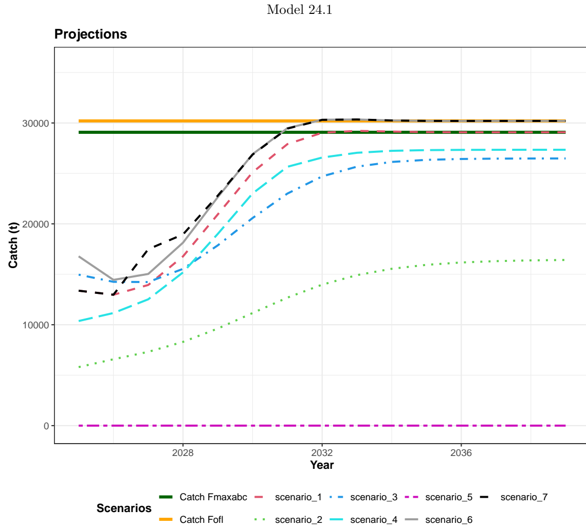
Figure 2A.37: Catch under seven NPFMC projection scenarios for Model 24.1.
