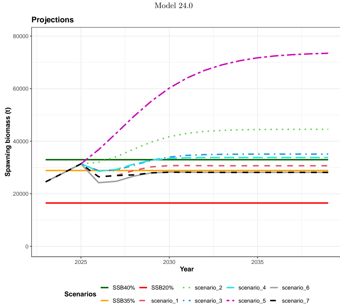
Figure 2A.42: Projected spawning stock biomass under seven NPFMC projection scenarios for Model 24.0.
