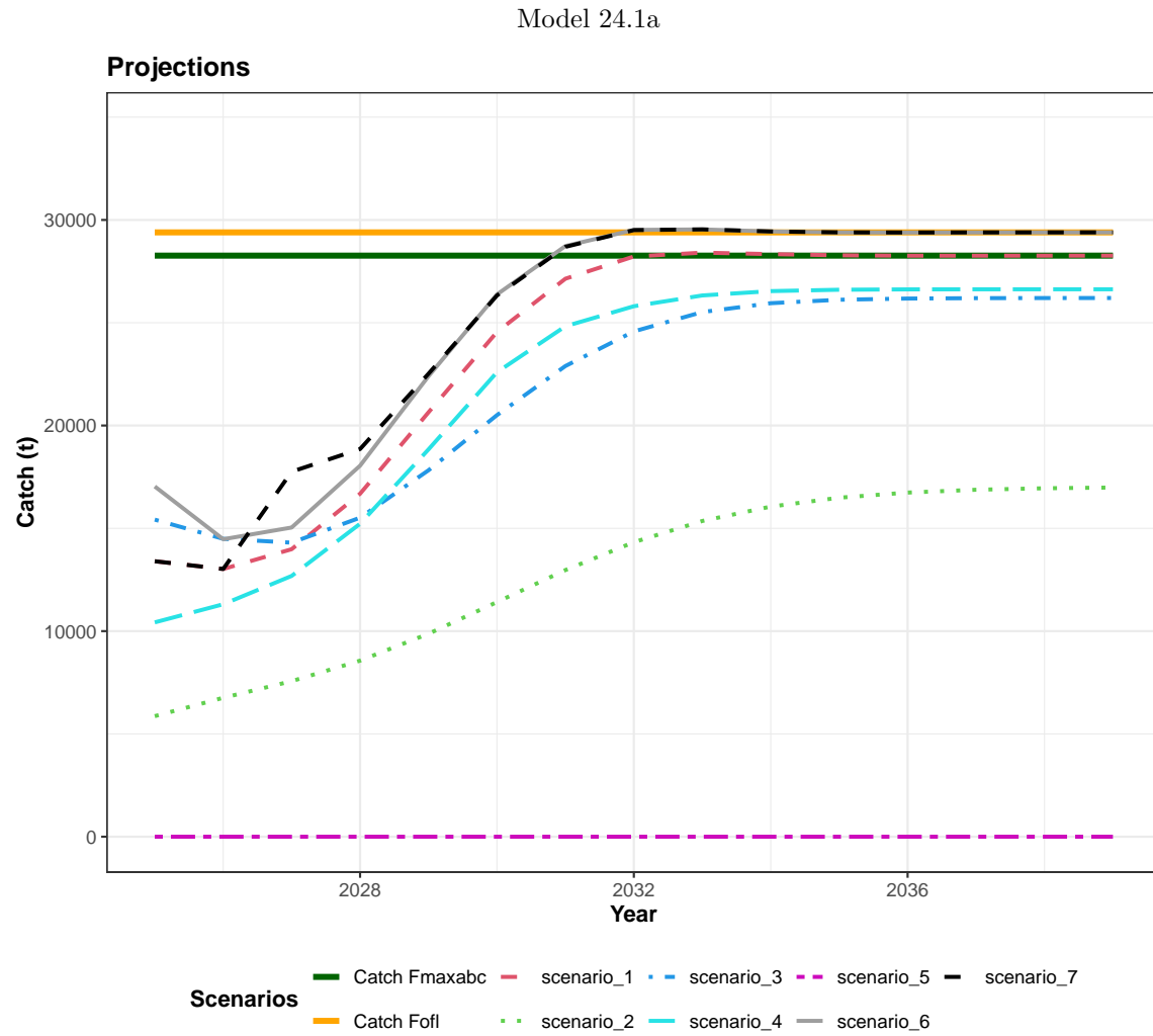
Figure 2A.38: Catch under seven NPFMC projection scenarios for Model 24.1a.
