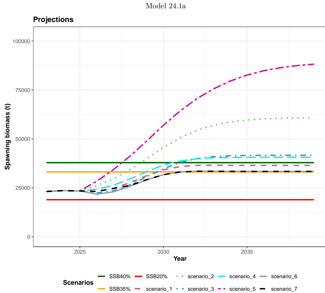
Figure 2A.41: Projected spawning stock biomass under seven NPFMC projection scenarios for Model 24.1a.
