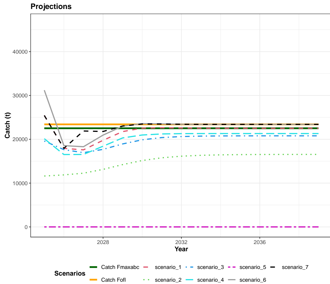
Figure 2A.39: Catch under seven NPFMC projection scenarios for Model 24.0.
