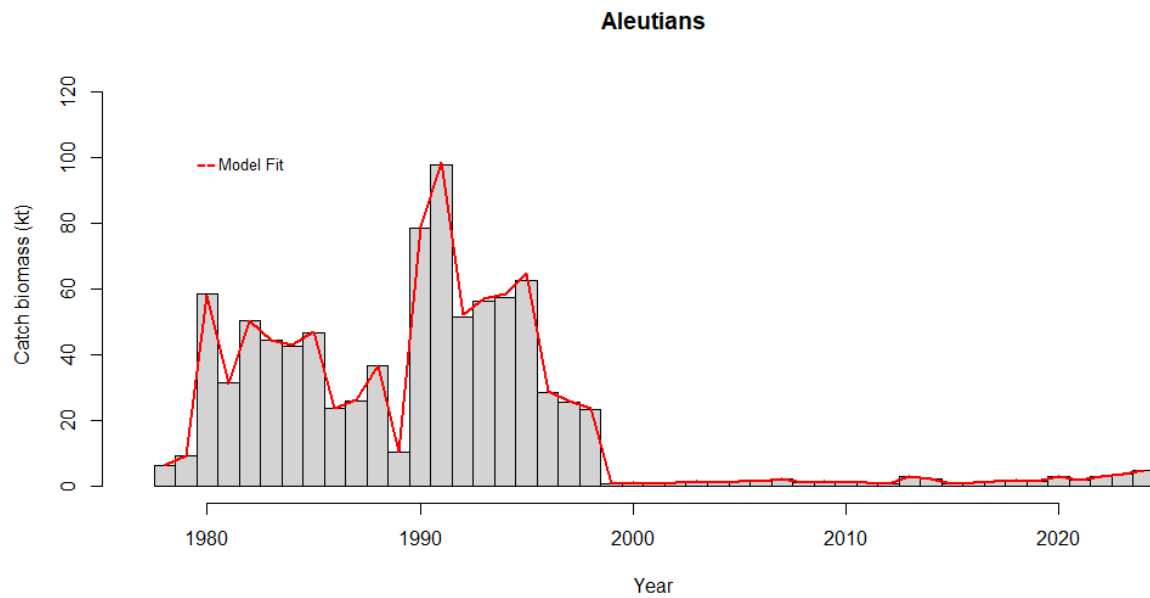
Figure 1A. 18 Fits to total catch in 1,000s of tons for AI pollock over time 1978-2024.
