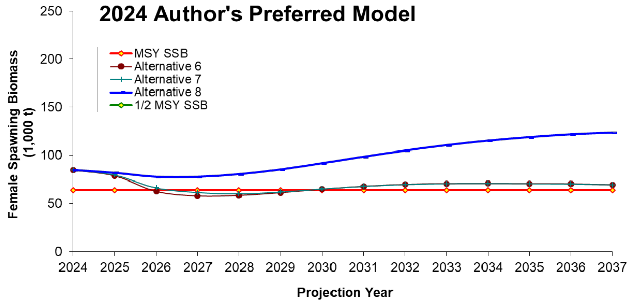
Figure 1A. 27 Authors' preferred Model 15.1 projected spawning biomass for MSY, \frac{1}{2} MSY, and Alternatives 6, 7, and 8 ABC scenarios from the authors' preferred model.
