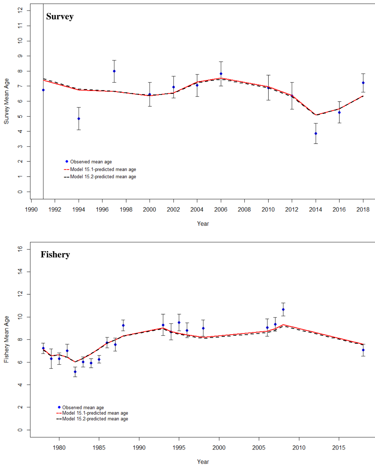
Figure 1A. 13 Observed mean age and model derived mean age from the AIBTS (top) and fishery catch at age data (bottom) for Model 15.1 and Model 15.2. The confidence intervals are adjusted by the multinomial sample sizes used in the models.
