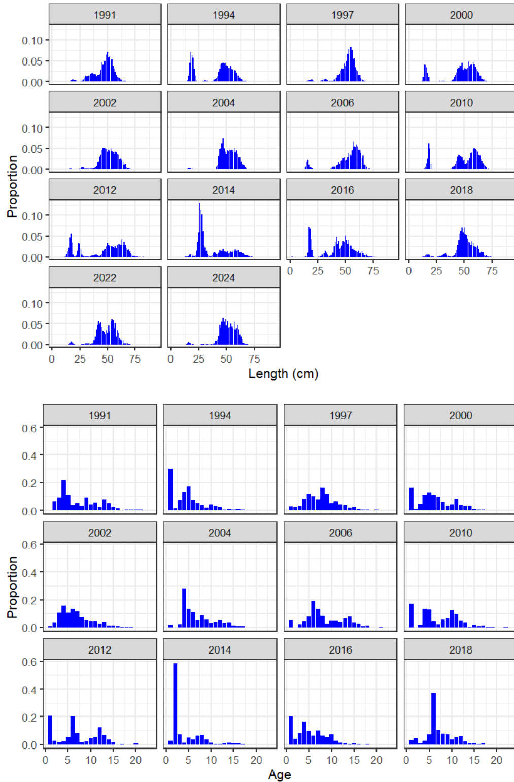
Figure 1A. 7 Distribution by (top) length and (bottom) Age for 1991-2024 Aleutian Islands bottom trawl surveys.
