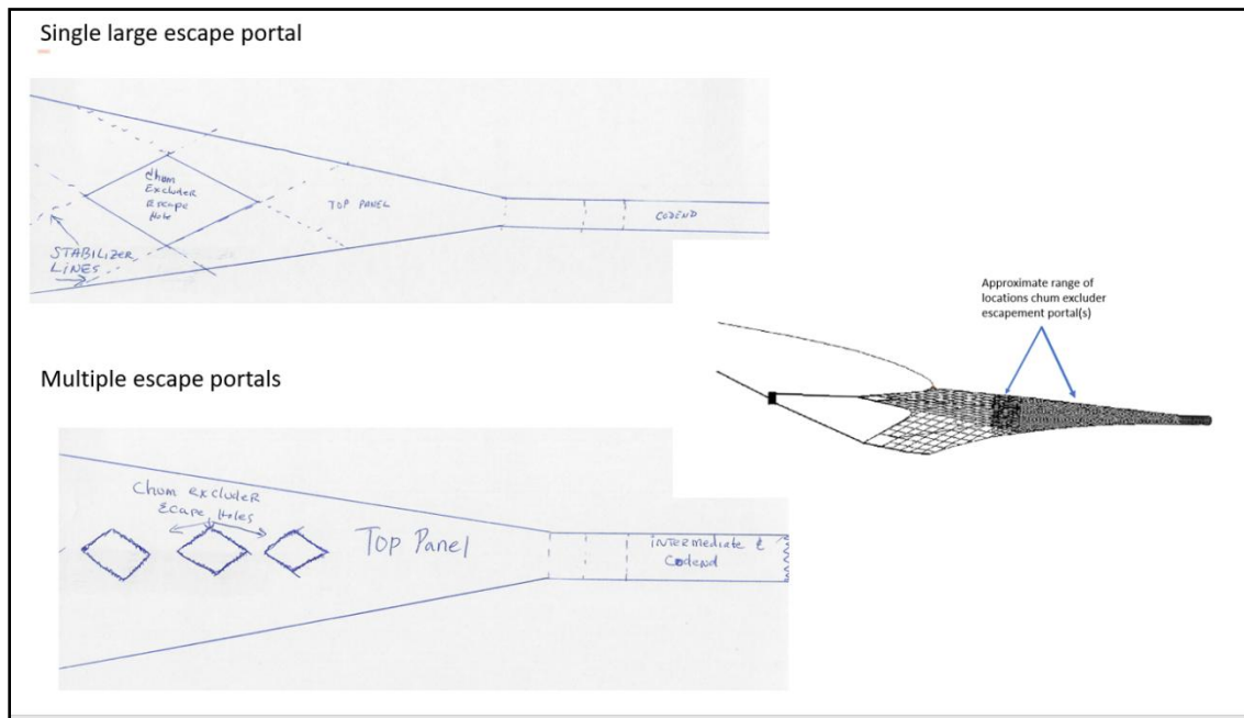
Figure 4. Conceptual design for a chum excluder with large escape portal(s) in the upper forward panel.
