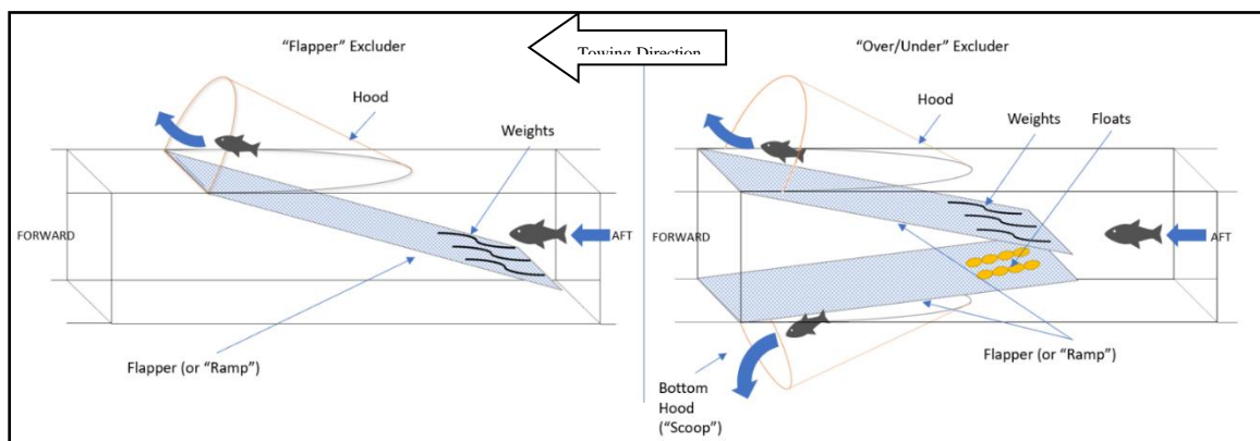
Figure 1. Single panel (Flapper) and Double panel (Over and Under) excluder designs
