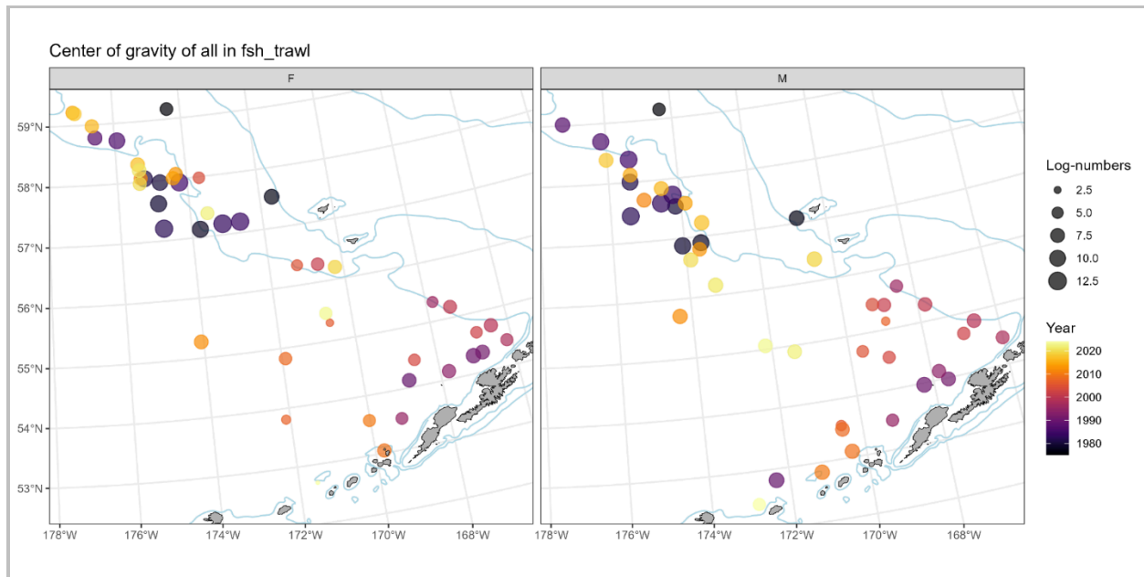
Figure 5.9 Mean annual center of gravity of the trawl fishery for Greenland turbot by sex. The size of the bubbles indicates the log-numbers of fished individuals, colors indicate the year.
