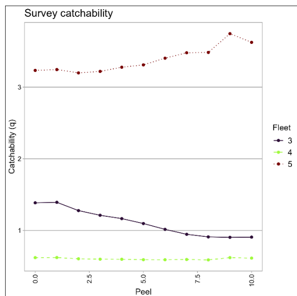
Figure 5.34 Retrospective plots for alternative model 24.2a as an example of the retrospective patterns in the alternative models. a) Female spawning biomass (full time series) b) female spawning biomass (last 10 years of the model), and c) survey catchability where Fleet 3 ~ EBS shelf bottom trawl survey, fleet 4 ~ EBS slope bottom trawl survey, and fleet 5 ~ AFSC longline survey.
