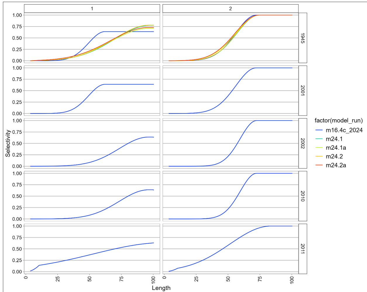
Figure 5.30 Time-varying selectivity at size by sex for the EBS slope bottom trawl survey. The estimated selectivity for Models 24.1, 24.1a, 24.2, and 24.2a was not time-varying and plotted in the 1945 facet. The value 1 represents females and 2 represents males.
