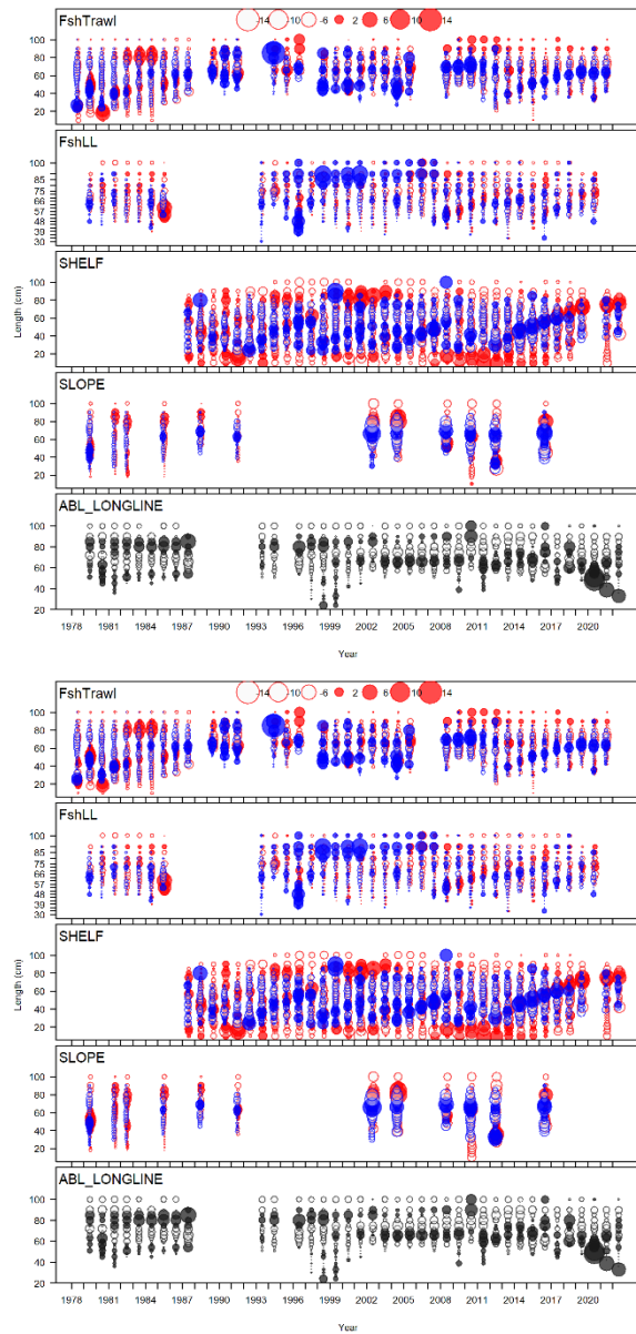
Figure 19. Pearson residuals across fleets for individual model runs indicated by the alpha-numeric label. Blue bubbles represent males, red represents females, and black represents combined sex.
