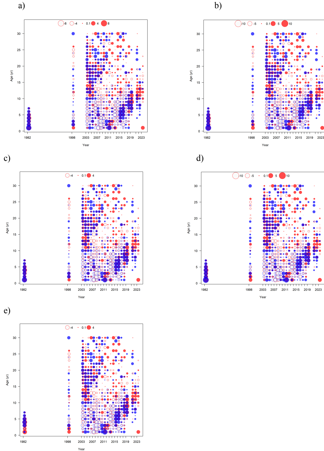
Figure 5.22. a) The standardized residuals for the fit to the mean length at age data from a) Model 16.4c and b) Model 24.1, and c) Model 24.1a, d) 24.2, and e) 24.2a. The closed bubbles are positive residuals (underestimation) and open bubbles are negative residuals (overestimation). Red bubbles are female and blue are male.
