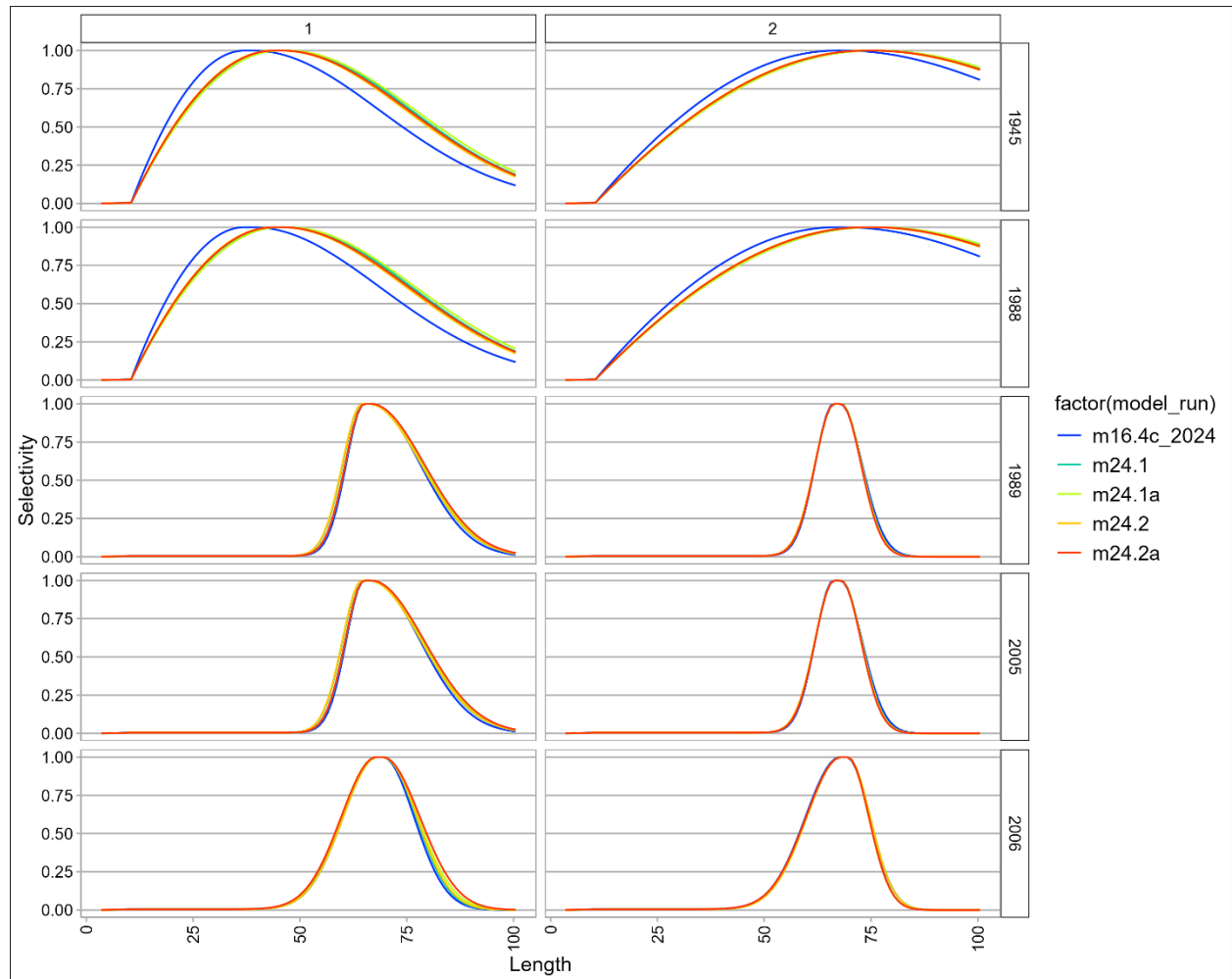
Figure 5.27. Time-varying selectivity at size for the trawl fishery for both sexes. The value 1 represents females and 2 represents males.
