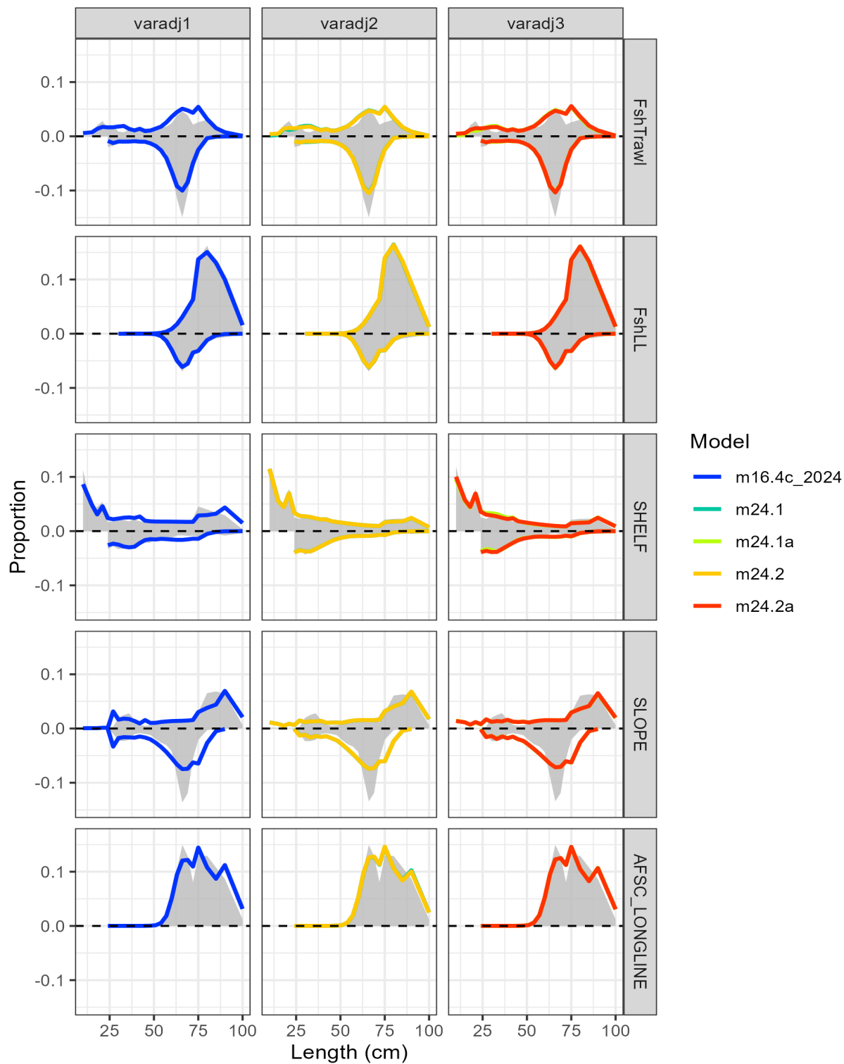
Figure 5.25. Fit to the aggregated length composition data by fleet, model, and assumption about the combination of input sample size and variance adjustment. Varadj2 represents the afscISS sample size for bottom trawl surveys reported in Table 5.14 and no variance adjustment, varadj3 represents the afscISS sample size and m16.4c variance adjustments inputs.
