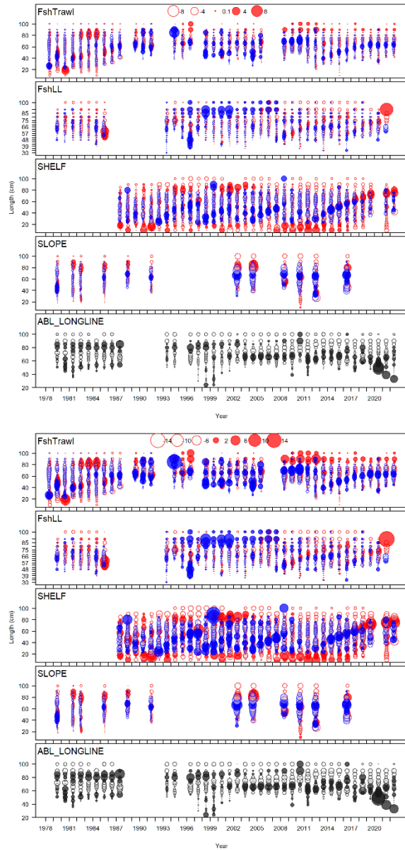
Figure 15. Pearson residuals across fleets for individual model runs indicated by the alpha-numeric label. Blue bubbles represent males, red represents females, and black represents combined sex.
