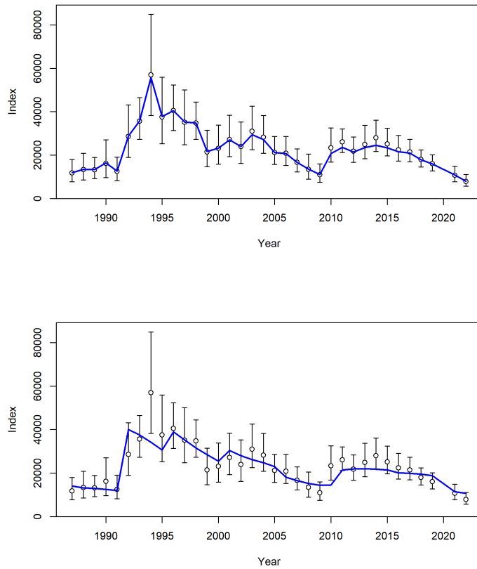
Figure 22. Fit to the EBS shelf bottom trawl survey when time blocks are removed (top), catchability is time-varying (middle), and ~5 year time blocks are implemented throughout the time series (bottom).
