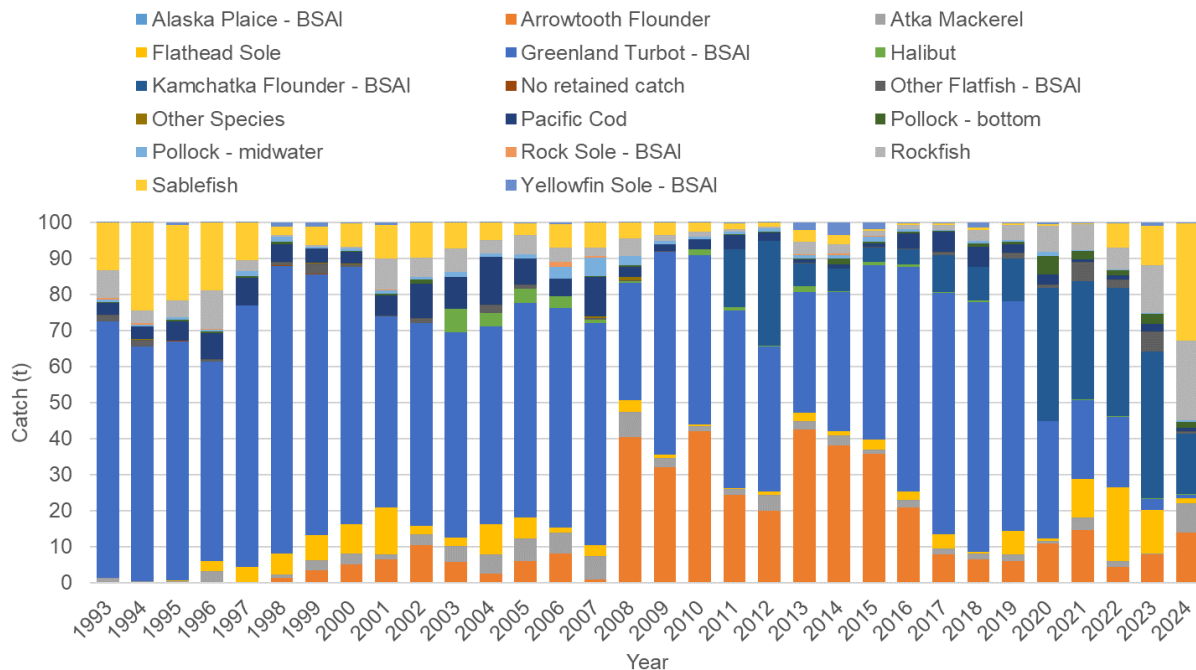
Figure 5.6. Catch per trip target species, 1993 – 2024.
