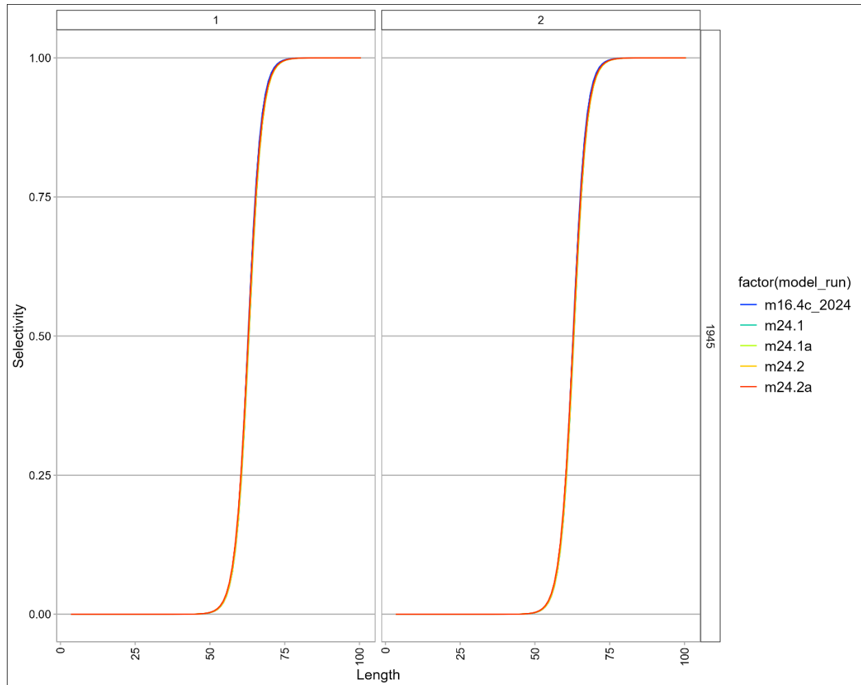
Figure 5.31 AFSC longline survey selectivity for females (1) and males (2).
