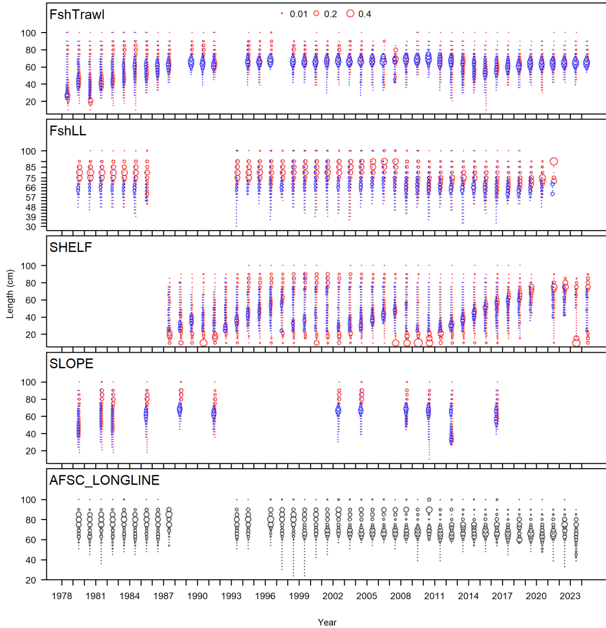
Figure 5.11. Greenland turbot size composition data from the trawl fishery, longline fishery, shelf survey, slope survey, and longline survey. Blue: males; red: females; black: combined sex.
