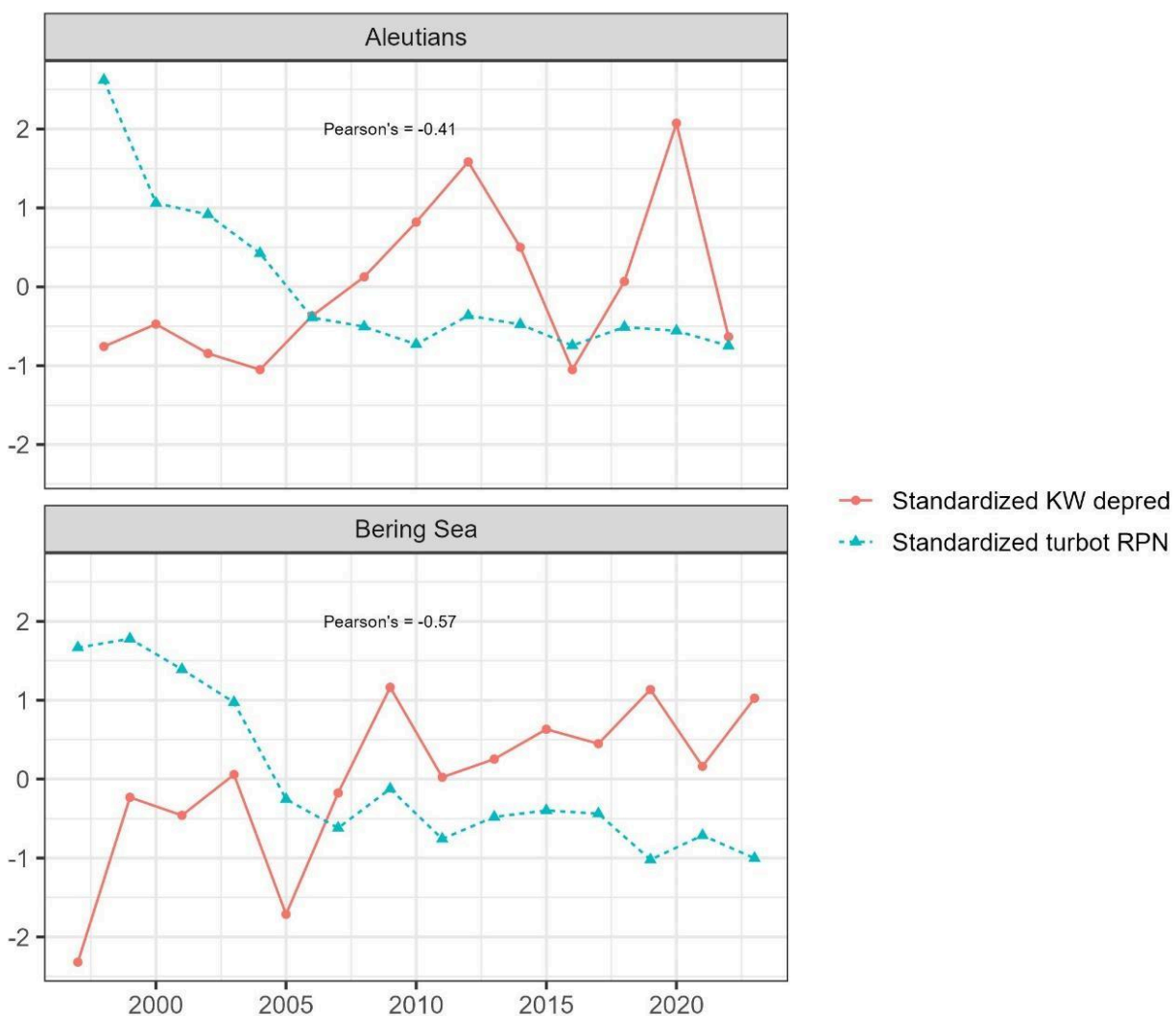
Figure 4. AFSC longline survey RPN estimates and killer whale depredation rates for the Aleutian Islands (top) and Bering Sea (bottom).
