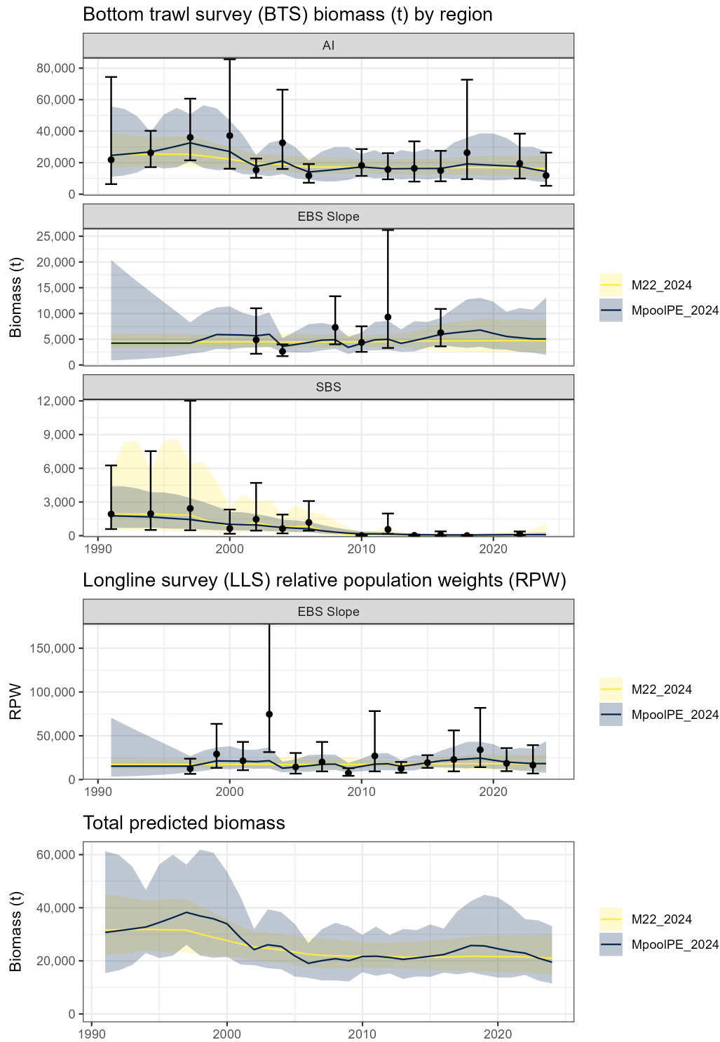
Figure 15.6 Sensitivity analysis comparing fits to the data and total predicted biomass between the recommended Model 22_2024 and a model with a single pooled process error (MpoolPE_2024).
