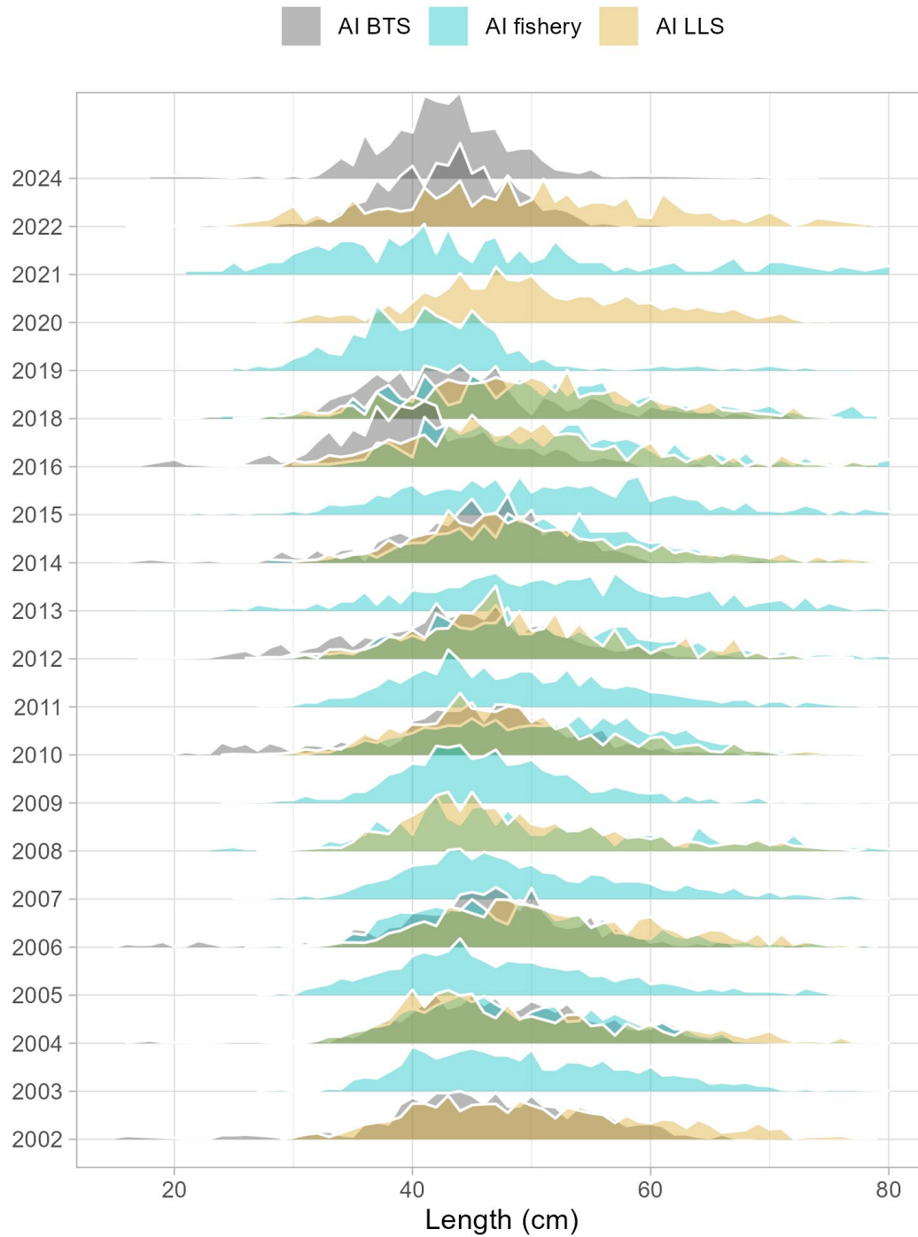
Figure 15.1a Length frequency data from the Aleutian Islands (AI) bottom trawl survey (BTS; grey), fishery (teal), and the Aleutian Islands longline survey (AI LLS; goldenrod) from 2002-present. Fishery data source: NMFS AFSC FMA Observer Debriefed Haul and Length tables. BTS data source: NMFS AFSC RACE AI Biomass and Length tables. LLS data source: NMFS AFSC ABL AI Area RPN tables.
