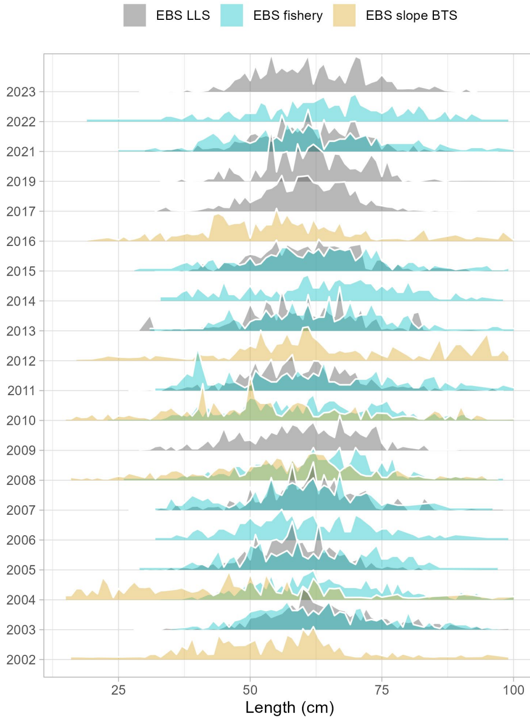
Figure 15.1b Length frequency data from the eastern Bering Sea longline survey (EBS LLS; grey), fishery (teal), and eastern Bering Sea slope bottom trawl survey (EBS slope BTS; goldenrod) from 2002-present. Fishery data source: NMFS AFSC FMA Observer Debriefed Haul and Length tables. BTS data source: NMFS AFSC RACE EBS slope Biomass and Length tables. LLS data source: NMFS AFSC ABL EBS slope Area RPN tables.
