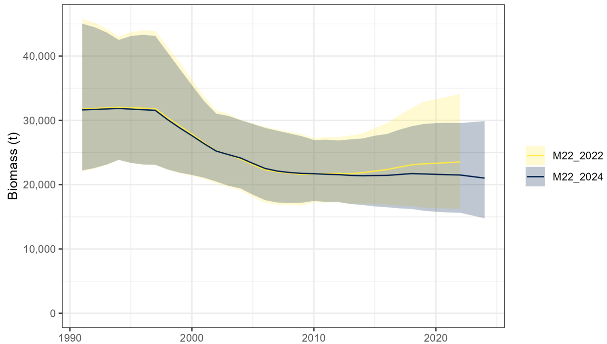
Figure 15.5 Total predicted biomass estimates for shortraker rockfish. Lines are the model predictions and shaded areas are the 95% confidence intervals from the random effects multi-area model with an additional survey (REMA) model. Results are shown for Model 22_2022 (yellow), the base model, and the Model 22_2024 (blue), the updated author-recommended model.
