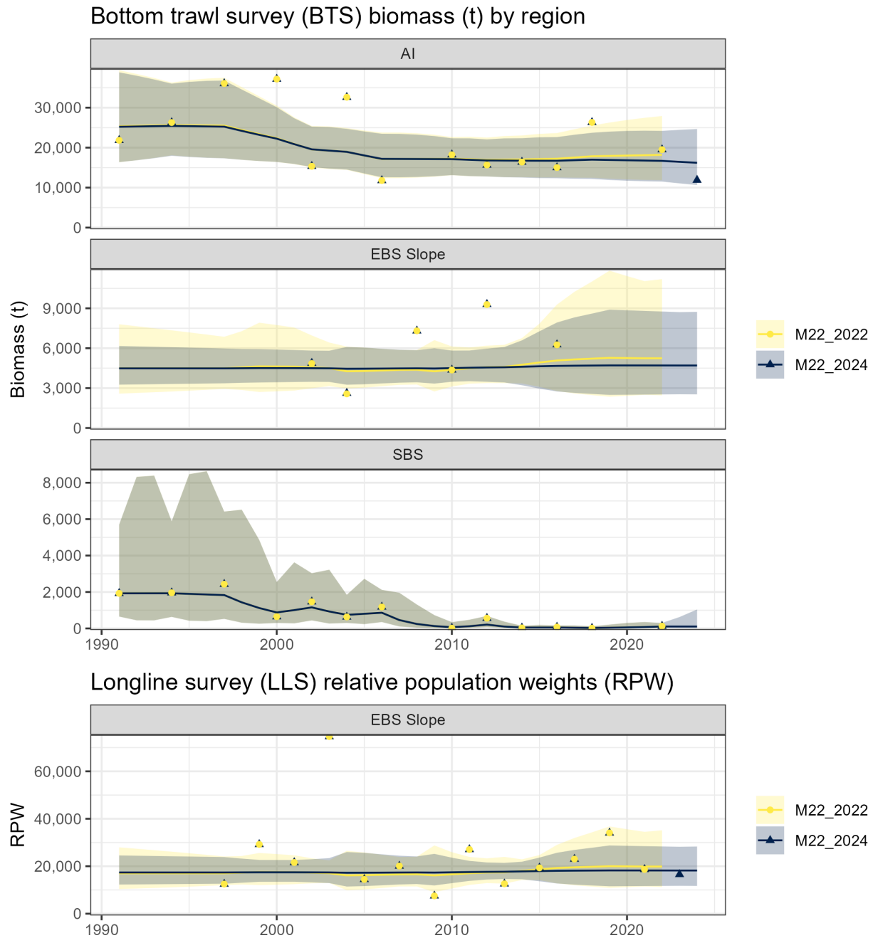
Figure 15.4 Observed biomass estimates and model fits to the Aleutian Islands (AI), eastern Bering Sea (EBS) slope, southeastern Bering Sea (SBS) bottom trawl surveys (BTS) by region (top three plots), fits to the EBS slope longline survey relative population weights (RPWs; bottom) for shortraker rockfish. Lines are the model predictions and shaded areas are the 95% confidence intervals from the random effects multi-area model with an additional survey (REMA) model. Results are shown for Model 22_2022 (yellow), the base model, and the Model 22_2024 (blue), the updated author-recommended model.
