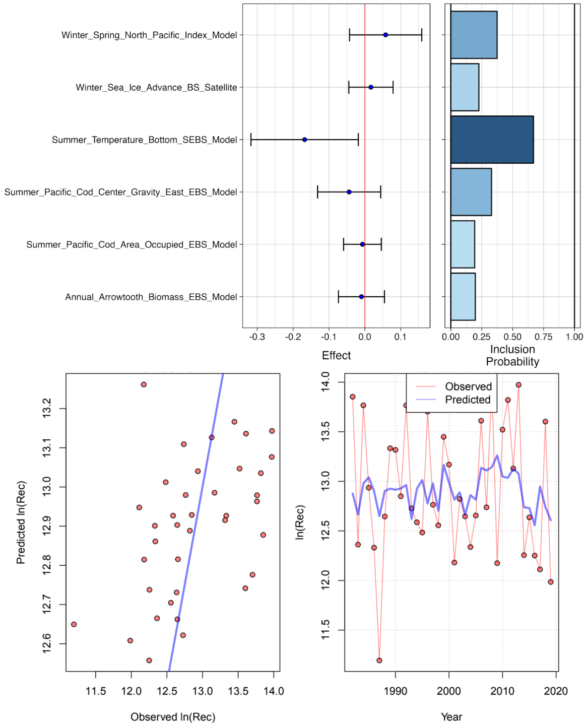
Figure 2.2.4: Bayesian adaptive sampling output showing the mean relationship and uncertainty ( \pm 1 SD) with log-transformed estimated EBS Pacific cod recruitment from the operational stock assessment model: the estimated effect (top left) and the marginal inclusion probabilities (top right) for each predictor variable of the subsetted covariate ecosystem indicator dataset. Output also includes model predicted fit (1:1 line, bottom left) and average fit across the abbreviated recruitment time series (1994-2019, bottom right)..
