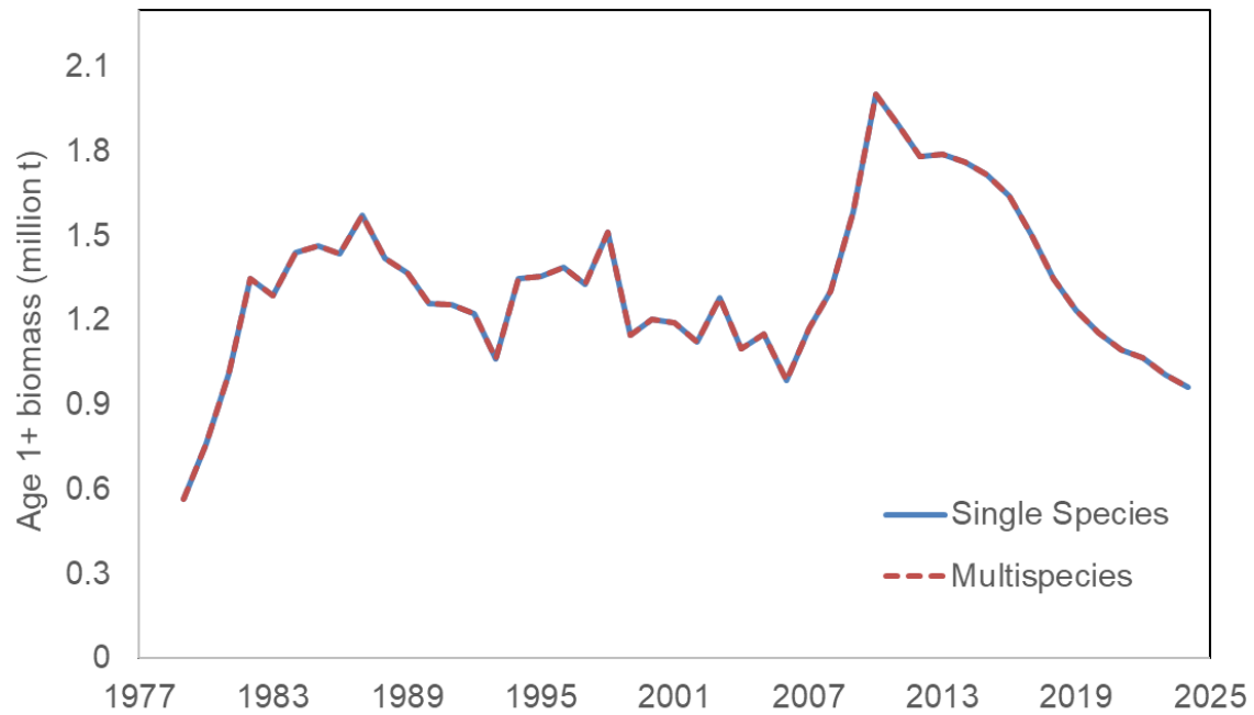
Figure 2.2.5: Age 1+ biomass for eastern Bering Sea Pacific cod from the most recent (Holsman et al., 2024) single species model (blue solid line) compared to the Climate- Enhanced, Age-based model with Temperature-specific Trophic Linkages and Energetics (CEATTLE) multispecies model (red dashed line).
