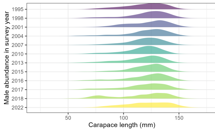
Figure 9: ADFG pot survey abundances by carapace length for male St. Matthew Island blue king crab from 1995 to 2022.
