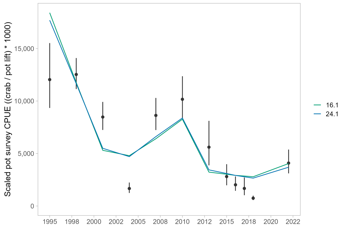
Figure 24: Comparisons of total (90+ mm CL) male pot survey CPUEs and model predictions for models 16.1 and 24.1. The error bars are plus and minus 2 standard deviations.
