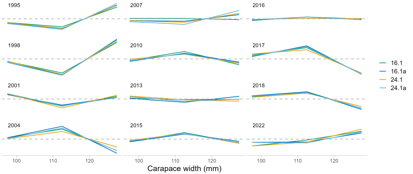
Figure 35: Line plots of residuals by size and year for the ADFG pot survey size composition data set for all models scenarios.
