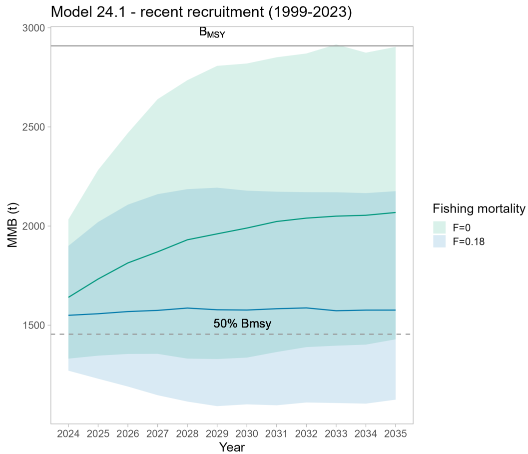
Figure 43: Mature male biomass (MMB) projections from model 24.1 for the next ten years using recent recruitment draws (1999 - 2023) and average bycatch levels from the last 5 years. Crab year “2024” represents Feb. 15, 2025. Solid colored lines represent mean projected MMB for each fishing mortality rate while shaded regions represent 0.05 to 0.95 quantiles. The solid horizontal line shows B_{MSY} while the dashed horizontal line shows MSST (the minimum stock size threshold, 0.5 * B_{MSY} ).
