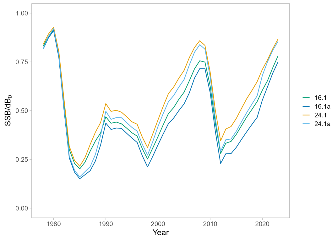
Figure 44: Comparison of spawning stock biomass (SSB) to the dynamic B_0 value (15 February, 1978-2023) for model 16.1, 16.1a, 24.1, and 24.1a.
