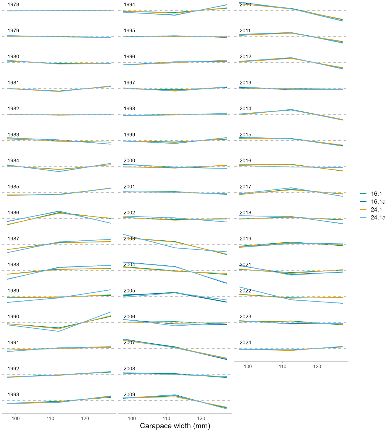
Figure 34: Line plots of residuals by size and year for the NMFS trawl survey size composition data set for all model scenarios.
