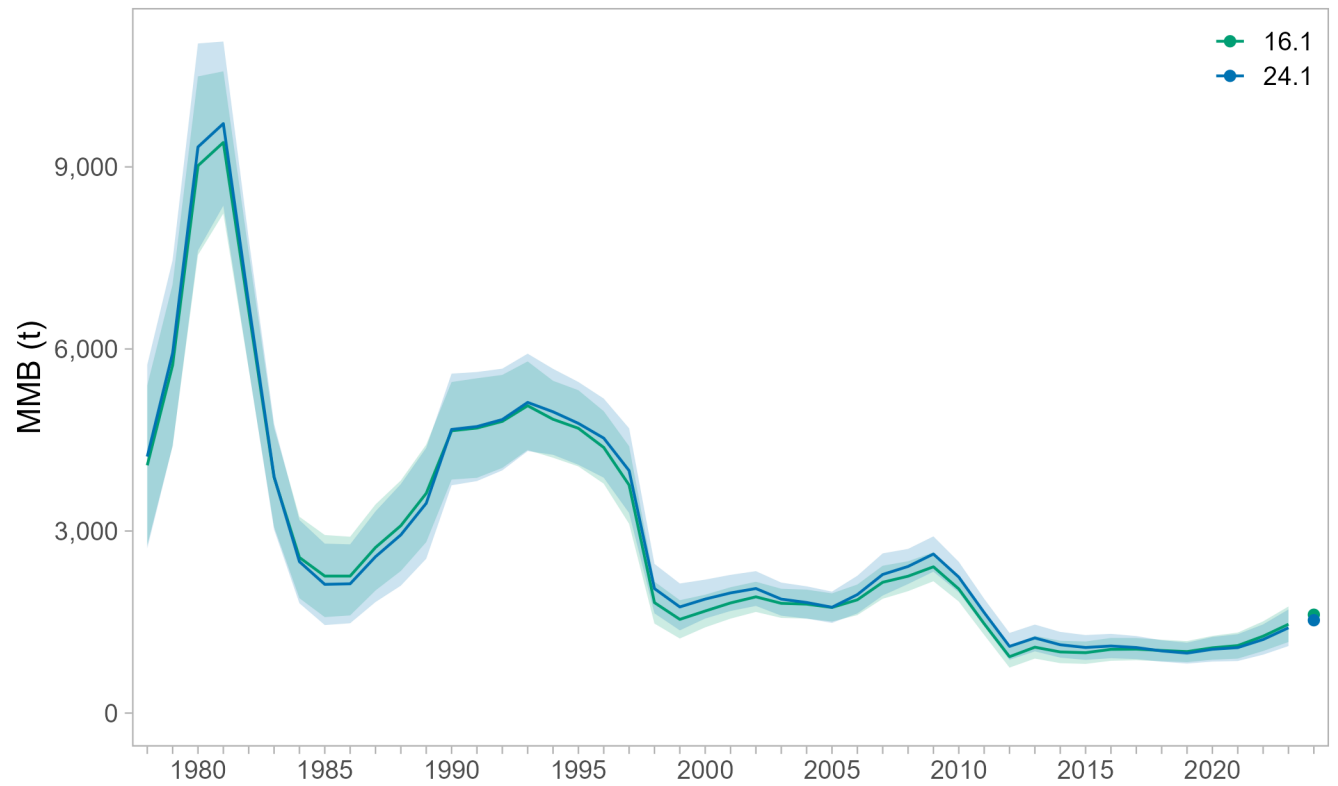
Figure 6: Comparisons of estimated mature male biomass (MMB) time series on 15 February (year + 1) during 1978-2024 for models 16.1 and 24.1. Points represent projected values for 2024/2025.
