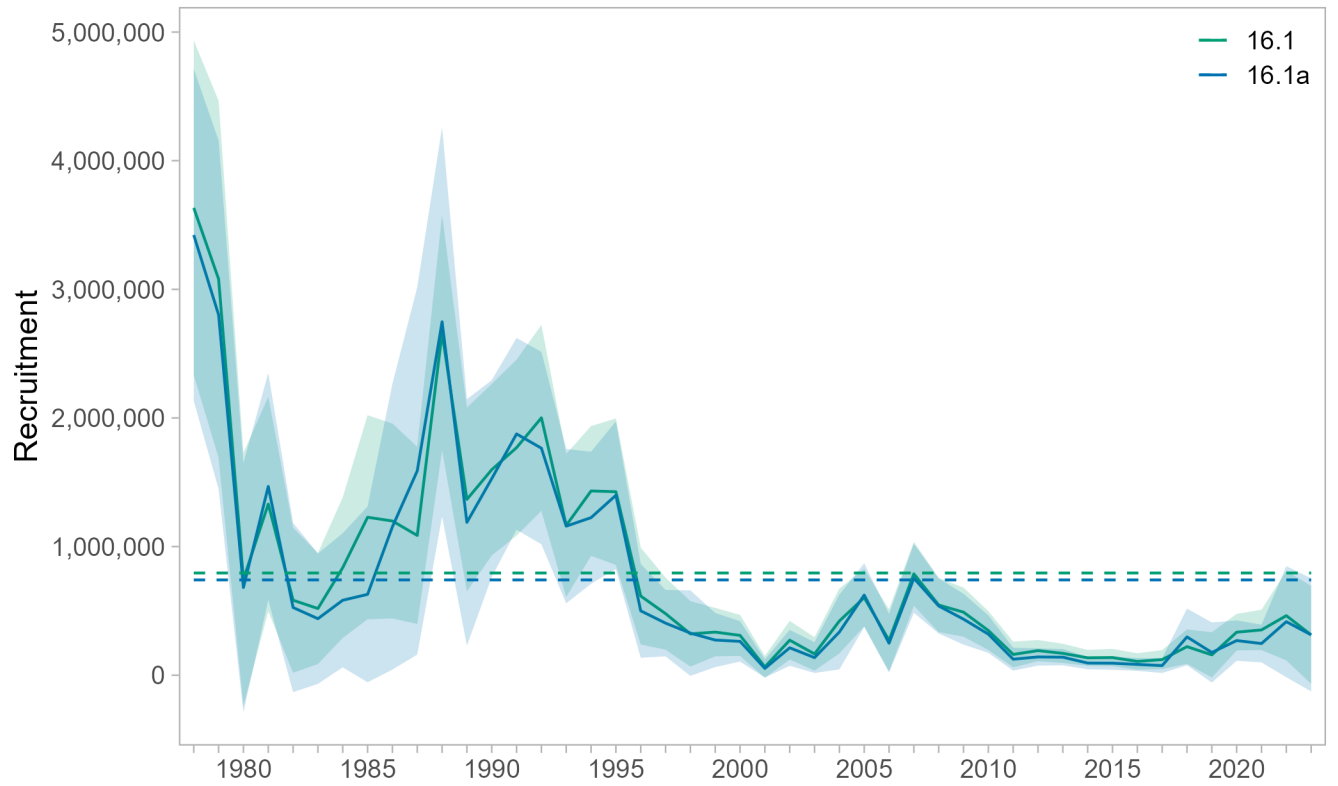
Figure 20: Estimated recruitment (in number of individuals) for 1979-2023 comparing models 16.1 and 16.1a. The dashed horizontal lines represent the estimate of the average recruitment parameter ( \bar{R} ) in each model scenario.
