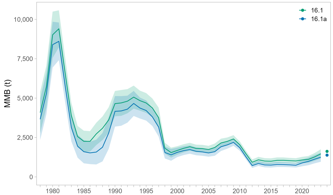
Figure 7: Comparisons of estimated mature male biomass (MMB) time series on 15 February (year + 1) during 1978-2024 for models 16.1 and 16.1a. Points represent projected values for 2024/2025.
