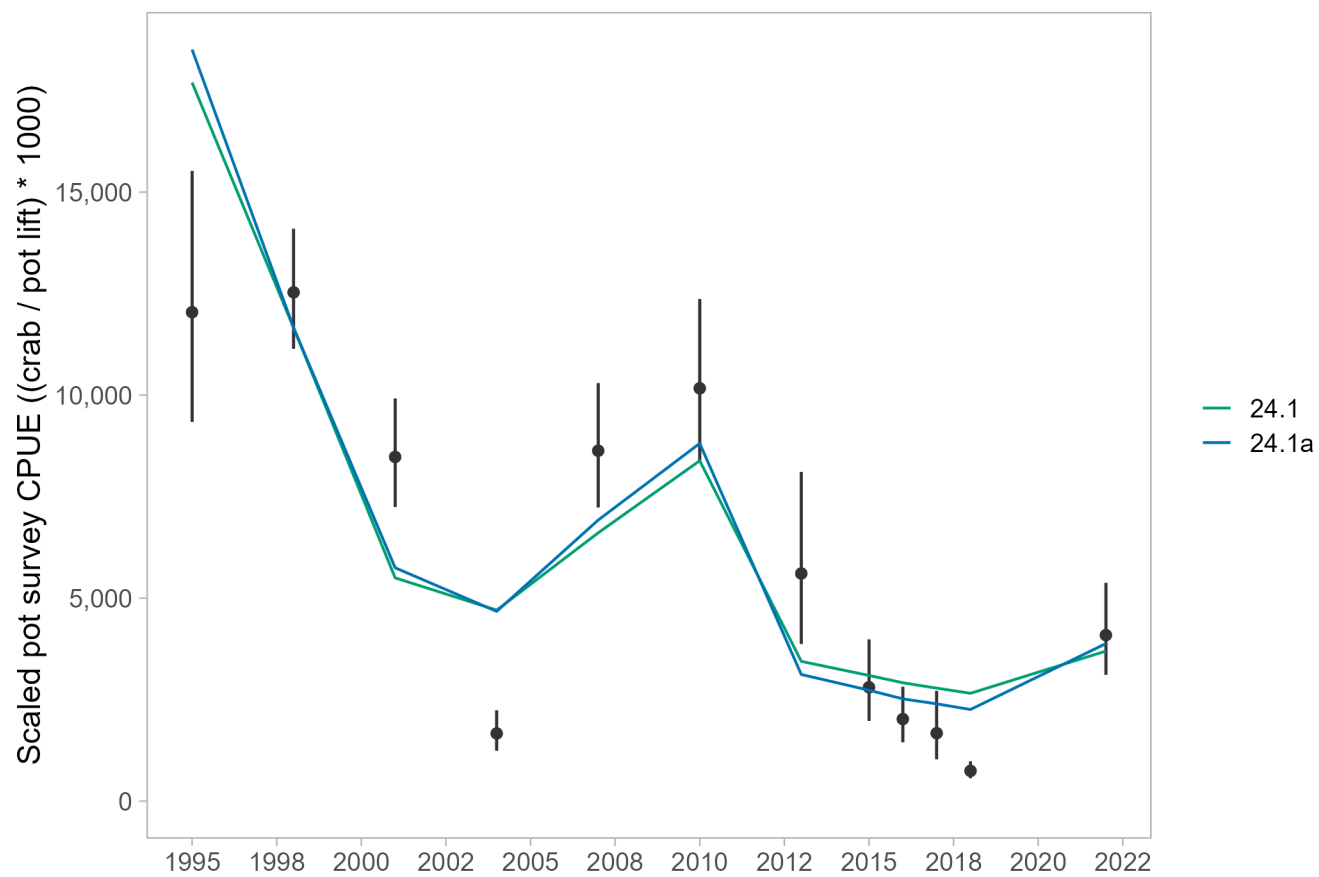
Figure 28: Comparisons of total (90+ mm CL) male pot survey CPUEs and model predictions for models 24.1 and 24.1a. The error bars are plus and minus 2 standard deviations.
