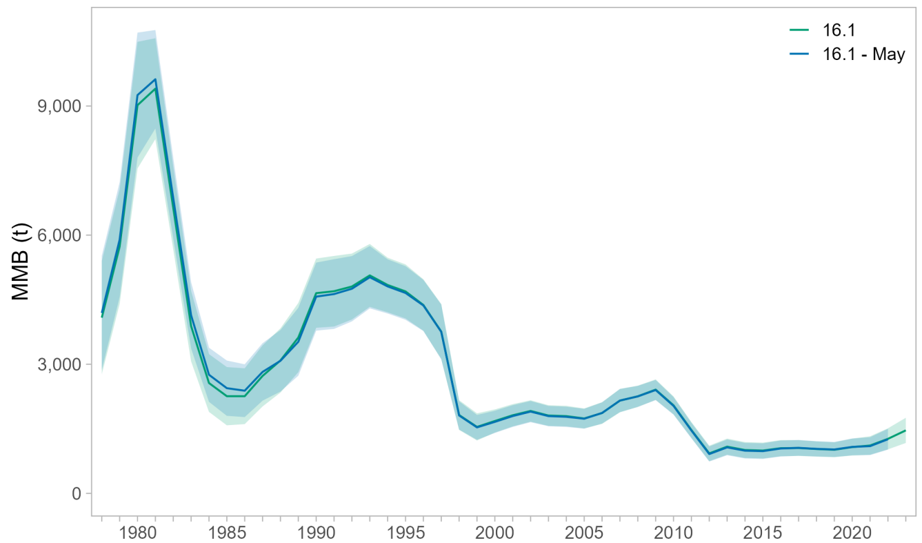
Figure 17: Estimated mature male biomass (MMB) over 1978-2024 from models 16.1 - May and 16.1; model 16.1 - May is the model recommended in May 2024 using the data then available and GMACS version 2.01.M.10, while model 16.1 is the same model translated to GMACS version 2.20.14 and updated with the data available in August 2024.
