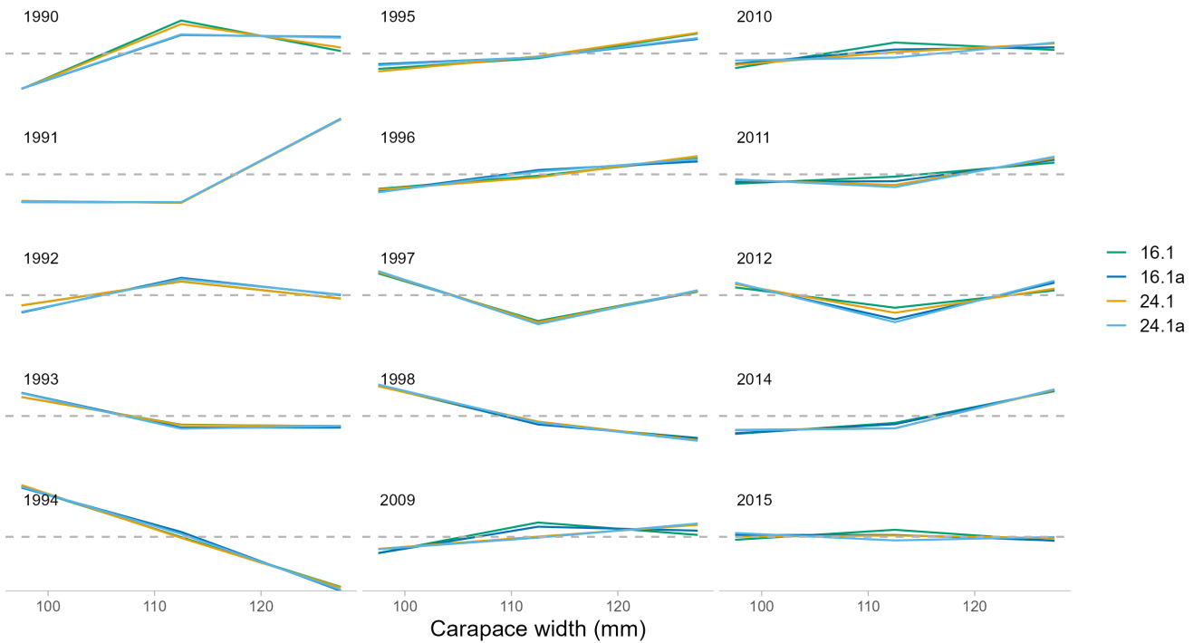
Figure 33: Line plots of residuals by size and year for the directed pot fishery size composition data set for all model scenarios.
